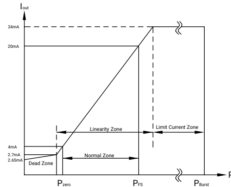
Output Current VS Pressure
